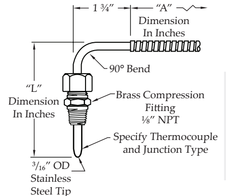
TCF90 - 90° Bend Thermocouple
